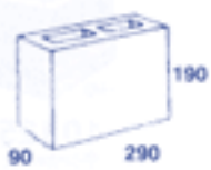
1002 Three Quarter
