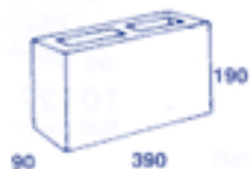
1001 Standard
