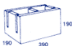
2020 Knock-out Bond Beam
