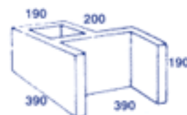
2060 Bonded Pilaster Half
