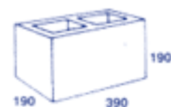
2001 Standard
