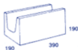
2012 Trough Beam
